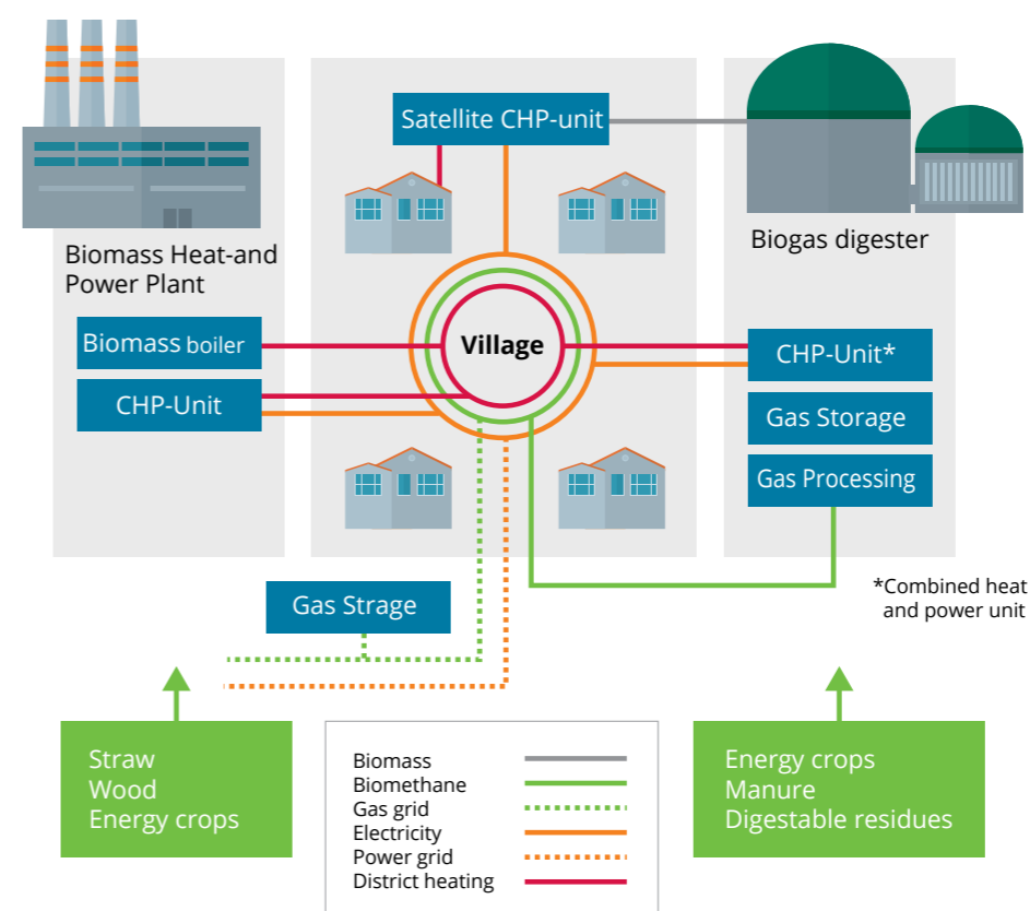
Figure 29 Material flows in a bioenergy village
