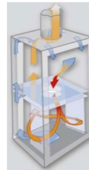
Figure 6: Air and exhaust gas flow in a twin-fire oven with optimised particle emissions
