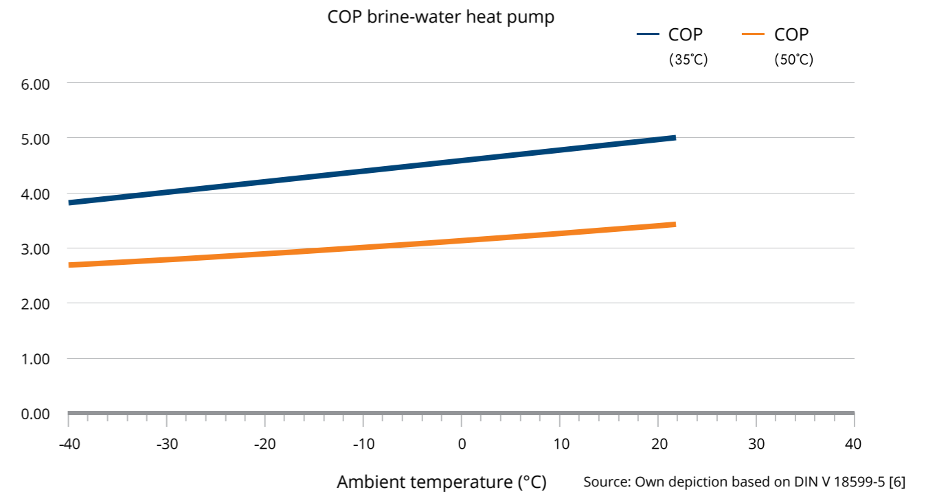
Figure 16: COP as a function of ambient temperature for different supply temperatures for GSHP
