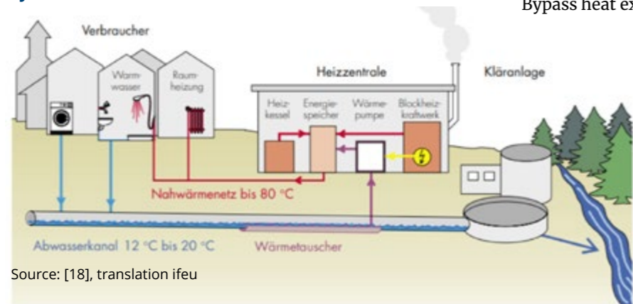
Figure 25: Principle of a waste water heat recovery system
