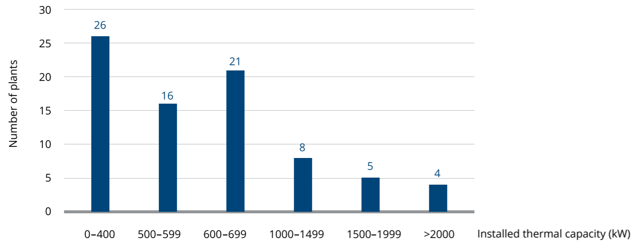
Figure 30 Installed thermal capacities (kW) of wood chip boilers in 80 bioenergy villages
