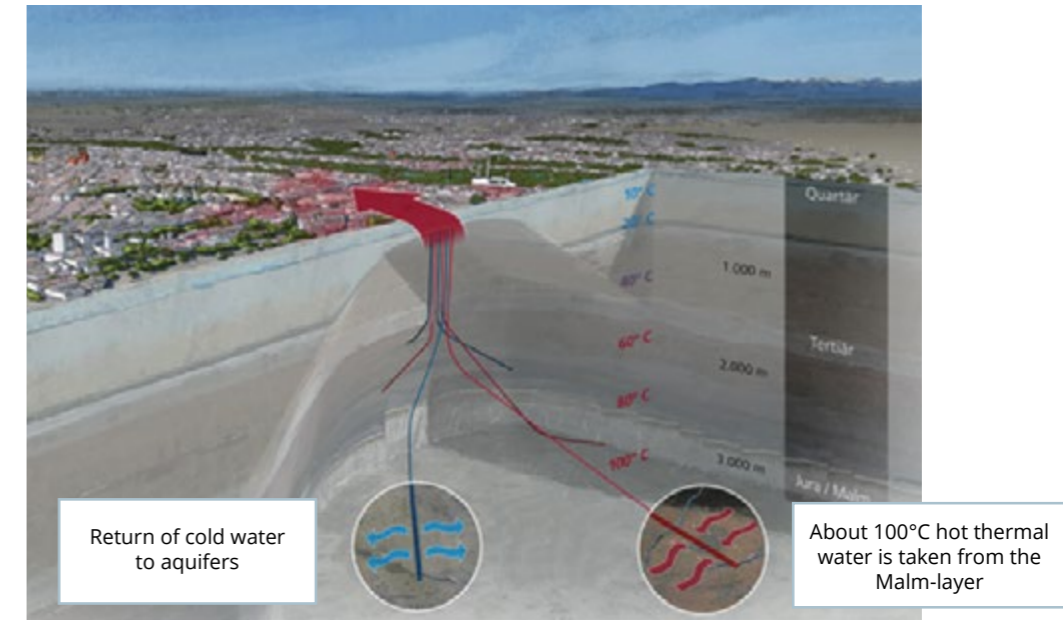
Figure 44: Deep geothermal plant in Munich
