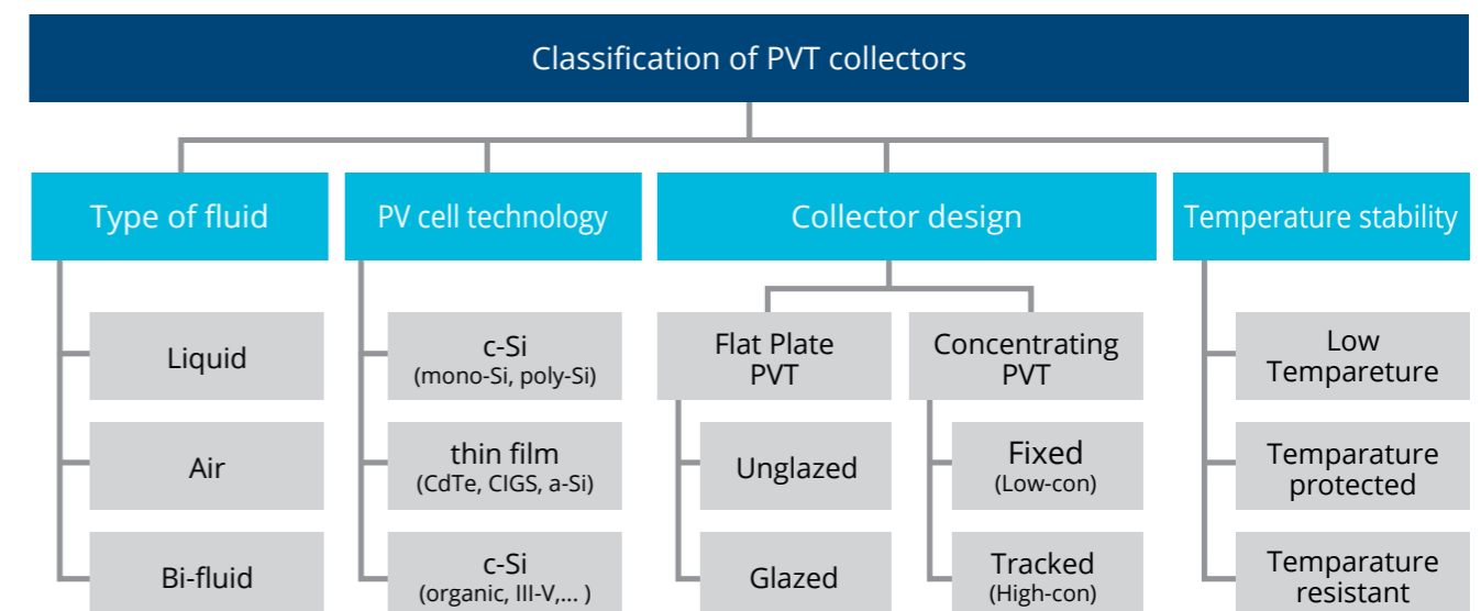
Figure 22: Classification of PVT collectors
