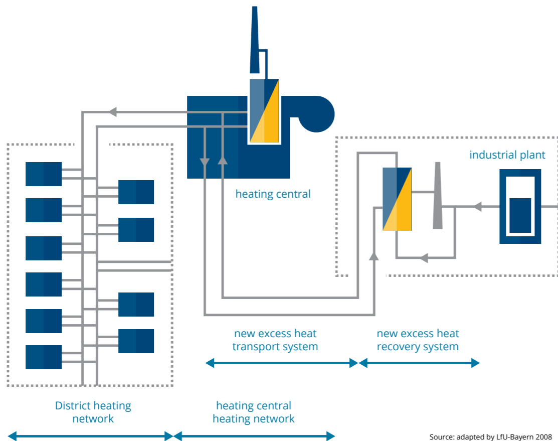
Figure 50: Schematic representation of excess heat recovery
