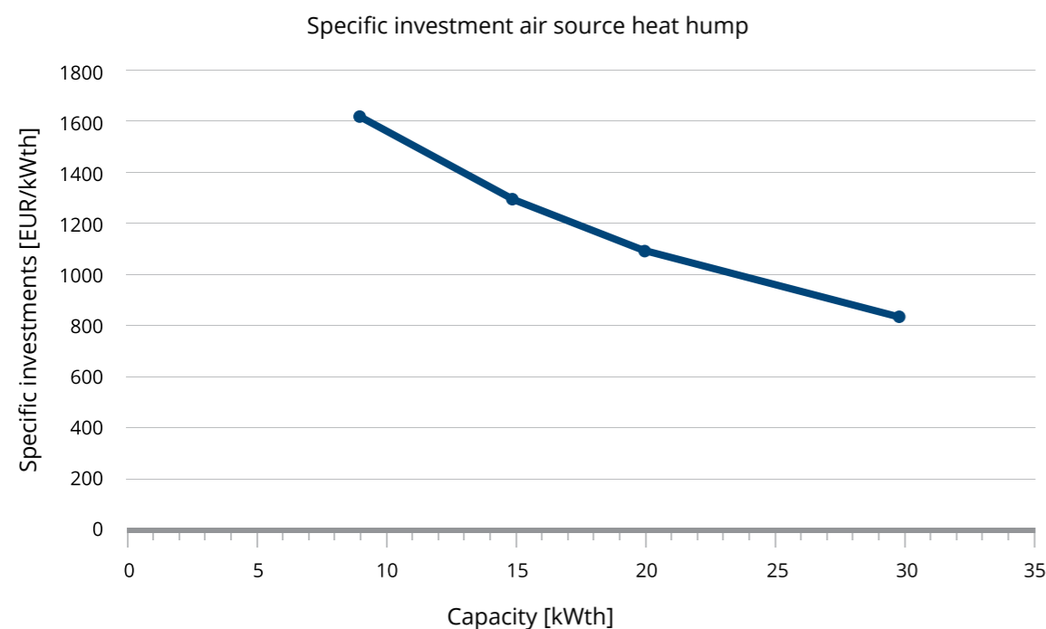
Figure 12: Specific investment costs of air source heat pumps in Germany
