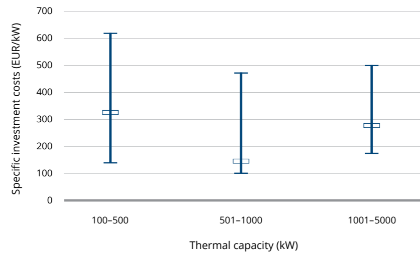
Figure 35 Specific investment costs of automatically stoked biomass-fired boilers, fully assembled, including ash removal, air and flue gas system, and flue gas cleaning
