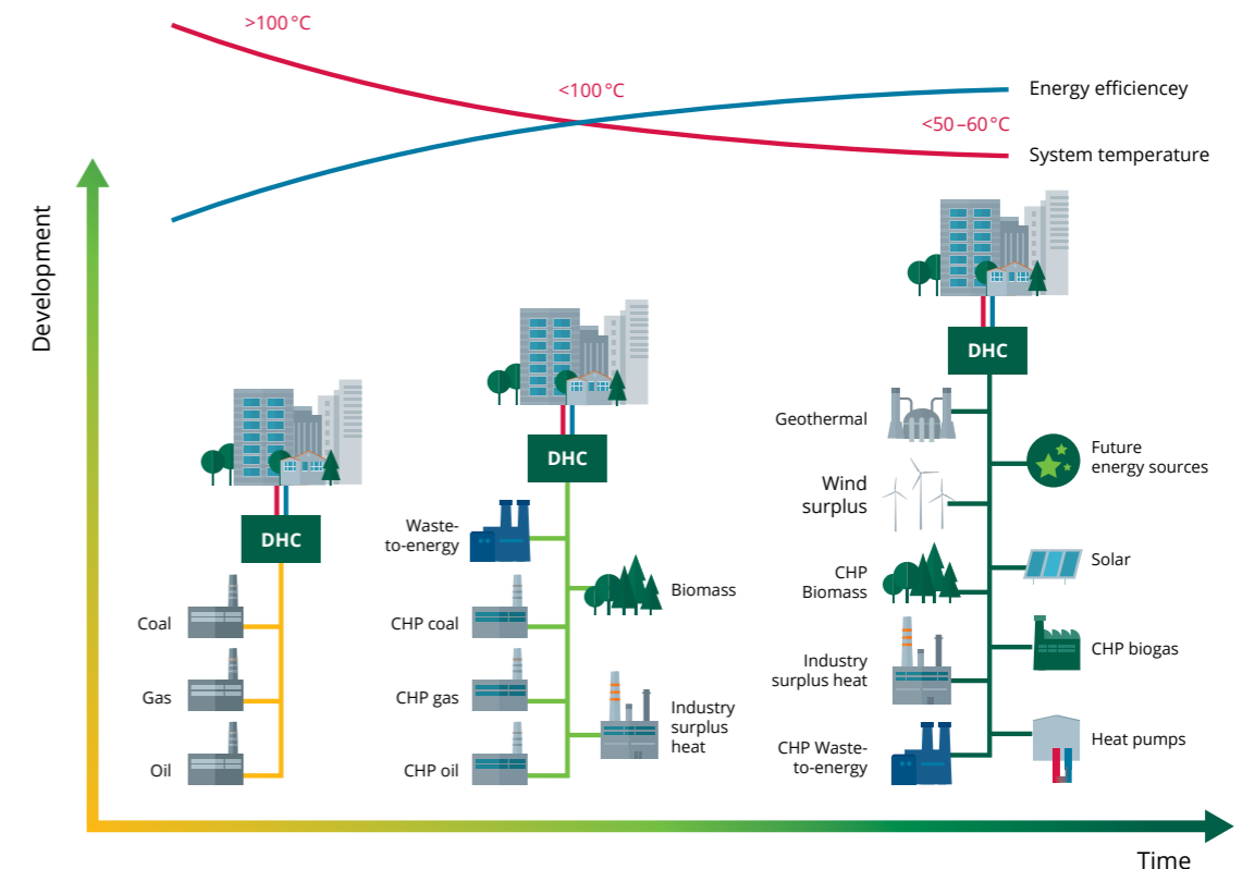
Figure 46: Evolution of district heating systems from fossil fuels to flexible multi-energy sustainable energy sources
