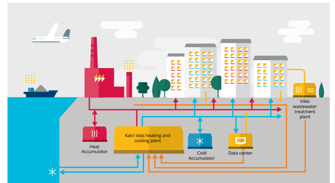
Figure 48: Combined Heat and Power (CHP)-based district heating/cooling (DHC) Helsinki
