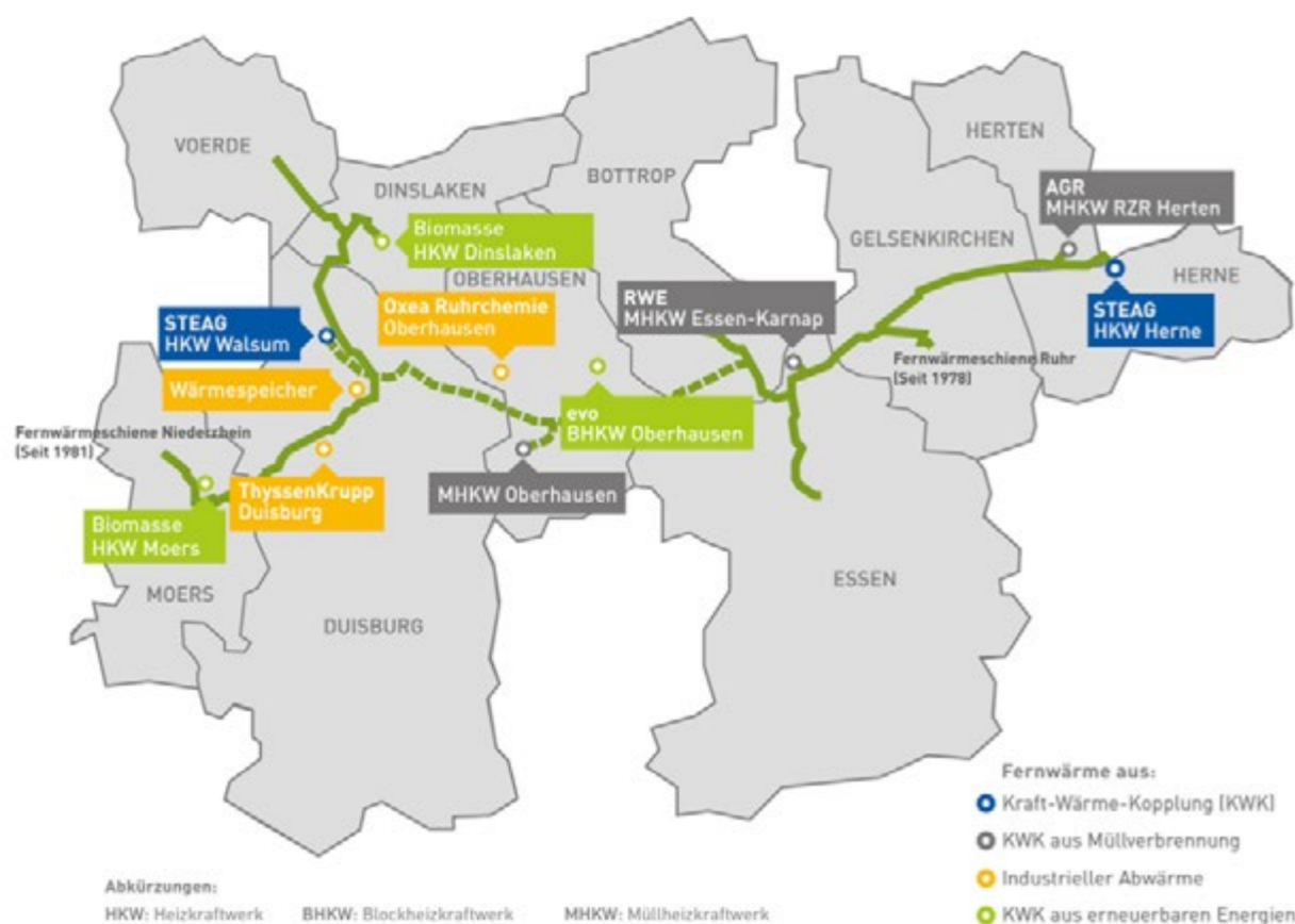
Figure 51: District heating rail Rhein-Ruhr
