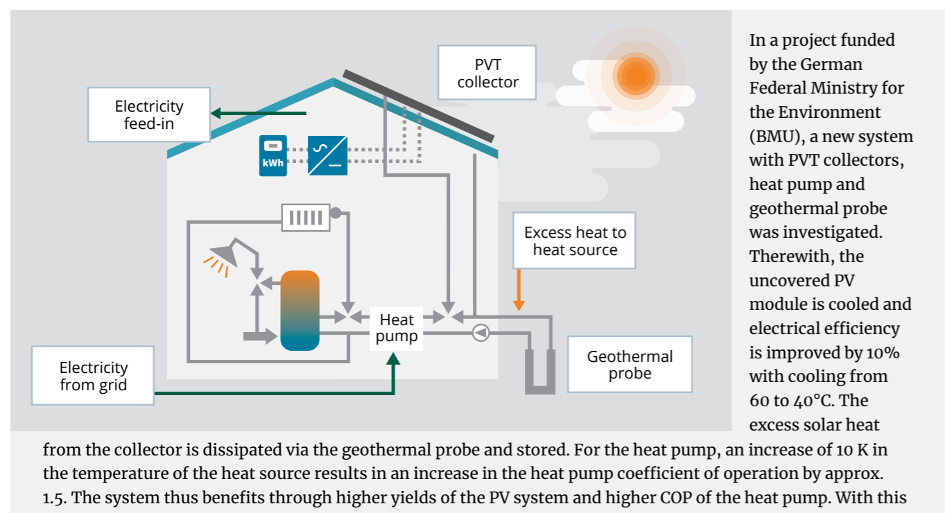
Figure 23: Storing excess heat from PV in geothermal probes
