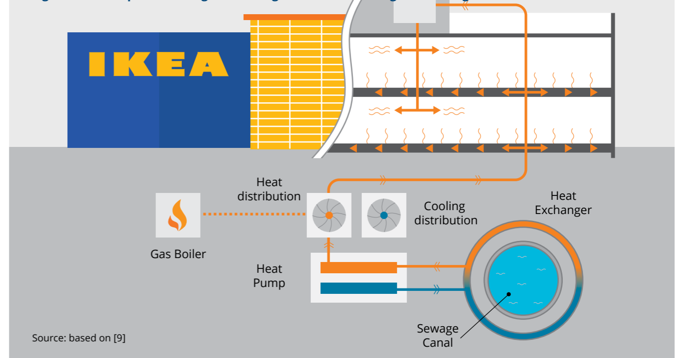
Figure 26: Concept for heating and cooling at IKEA Lichtenberg in Hamburg
