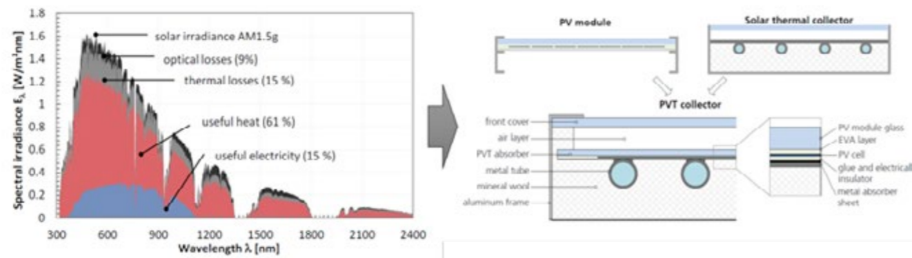
Figure 21: Useful energy for heating and electricity from solar irradiance and schematic depiction of PVT collector and heat pump
