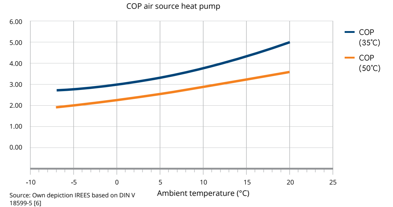
Figure 11: COP as a function of ambient temperature for different supply temperatures
