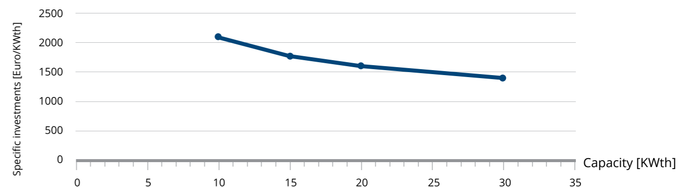
Figure 17: Specific investments of GSHP in Germany
