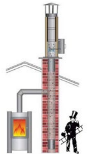
Figure 7: Filters for wood and other solid fuel stoves can be placed in the chimney or integrated into the stove
