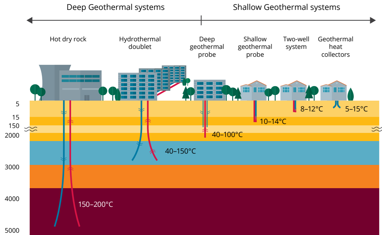
Figure 43: Different types of geothermal energy usage
