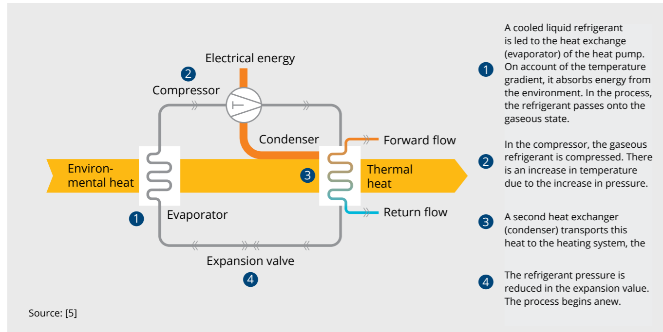
Figure 10: Principles of electric driven compression heat pump
