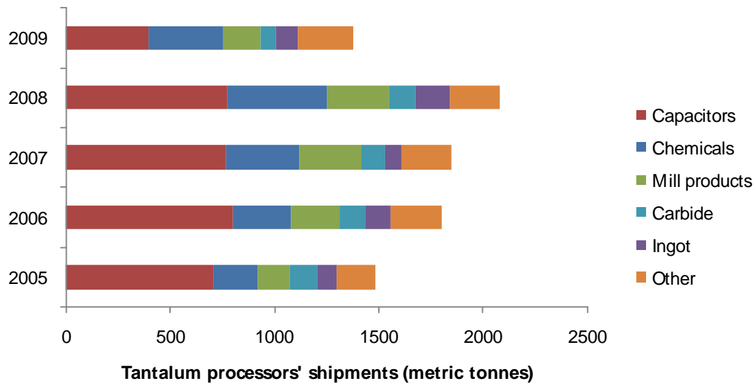
Figure 4: Tantalum processors' shipments (in metric tonnes of contained tantalum) between 2005 and 2009, as reported by the Tantalum-Niobium International Study Center (TIC). These figures are collected from TIC member companies and are thought to include most (but not all) shipments worldwide. Note that “capacitors” contains both capacitor-grade tantalum powder and tantalum wire while “mill products” excludes wire used for tantalum capacitors. Based on (Schwela 2010).
